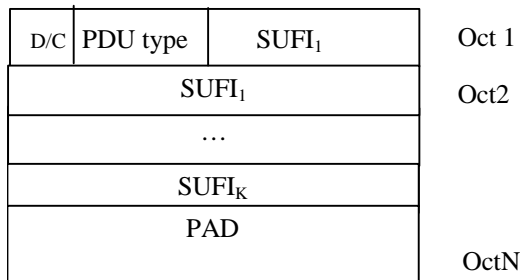
Figure 9.4: STATUS PDU
