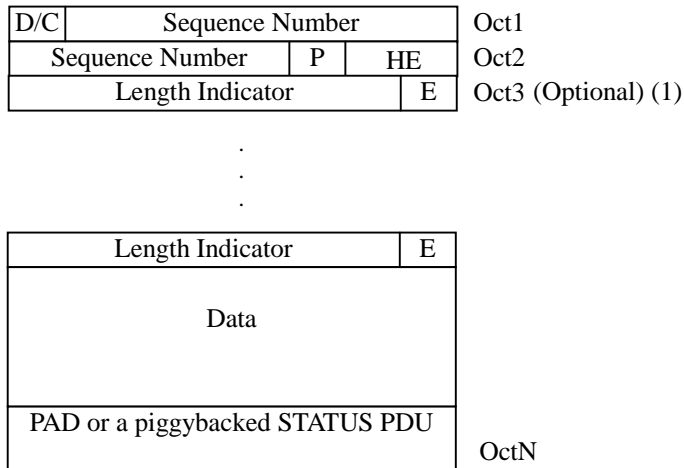
Figure 9.3: AMD PDU
