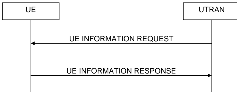
Figure 8.5.64.1-1: UE INFORMATION Procedure
