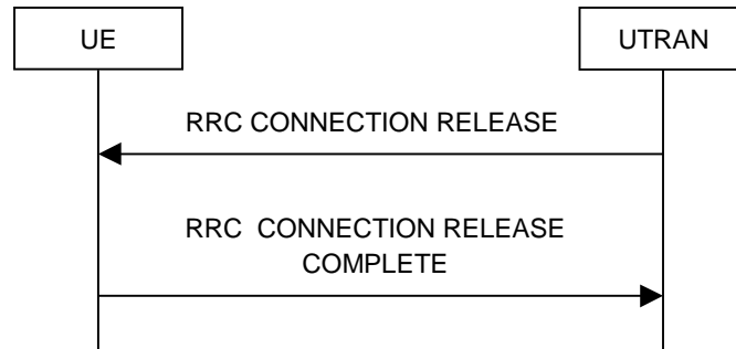
Figure 8.1.4-1: RRC Connection Release procedure on the DCCH
