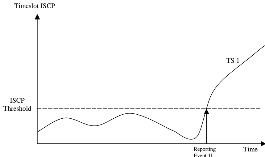
Figure 14.1.3.3-1: An ISCP value of a timeslot exceeds a certain threshold
