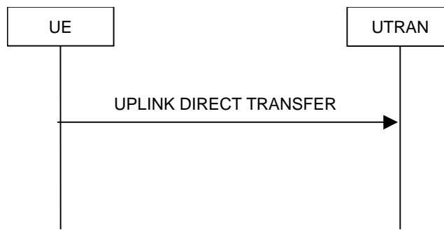
Figure 8.1.10-1: Uplink Direct transfer, normal flow
