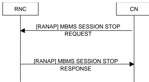
Figure 19: MBMS Session Stop procedure.
