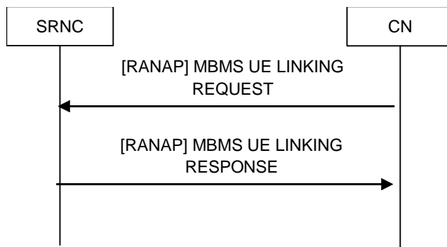
Figure 24: MBMS UE linking signalling flow
