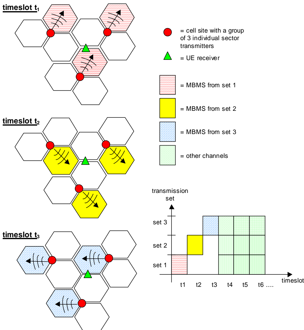
Figure 12: Example of non-time-coincident macro diversity transmission
