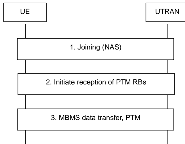
Figure 14: Joining with continuation of p-t-m
