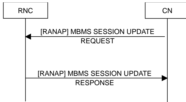
Figure 18: MBMS Session Update procedure. Successful operation.
