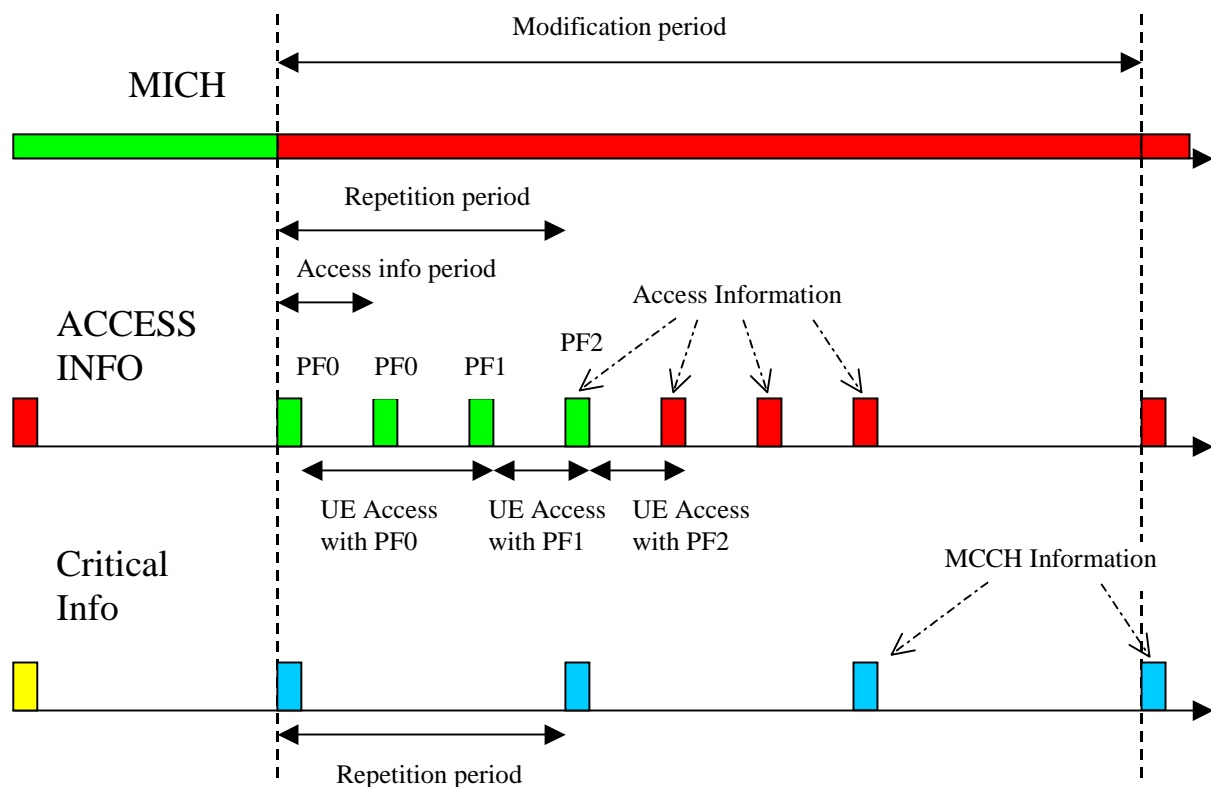
Figure 4: Illustration of Access Info period during MBMS counting
