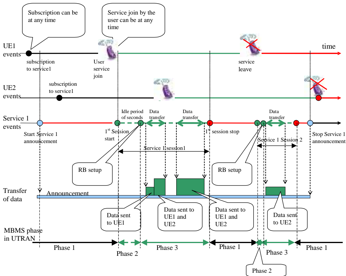
Figure 38: Timeline of MBMS Service
