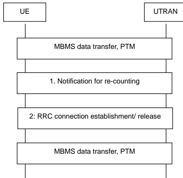
Figure 15: Recounting with continuation of p-t-m
