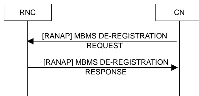
Figure 22: CN MBMS De-Registration procedure.
