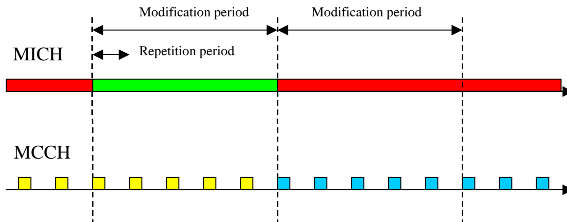
Figure 3: Illustration of MICH timing relative to Modification period
