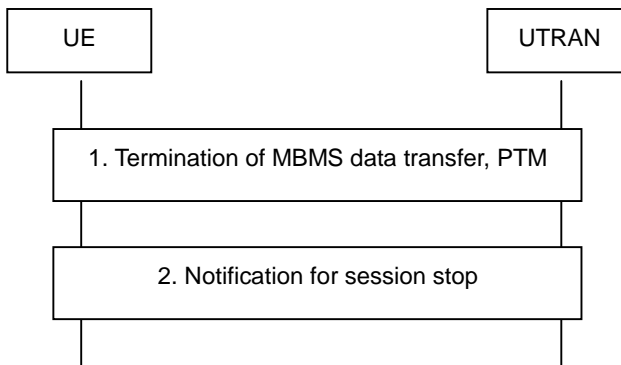
Figure 8.1.4: Session stop
