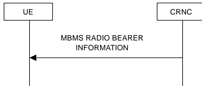
Figure 8.3.3: MBMS radio bearer information signalling flow
