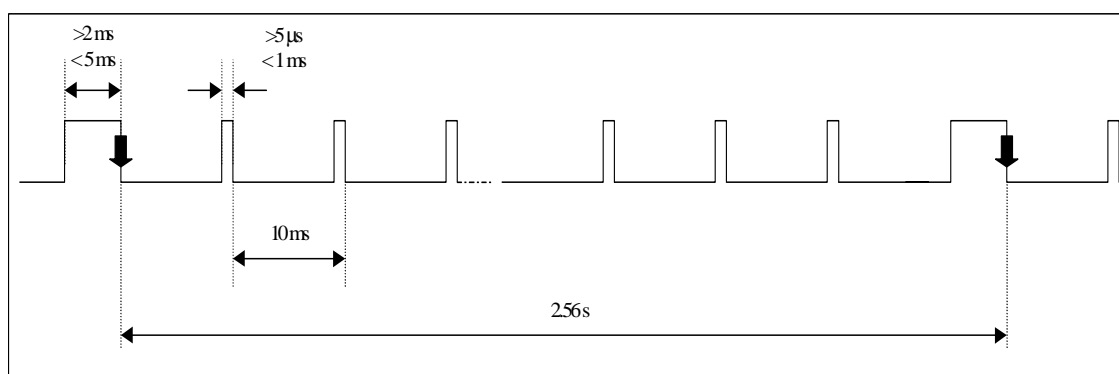
Figure 7: Synchronisation signal
