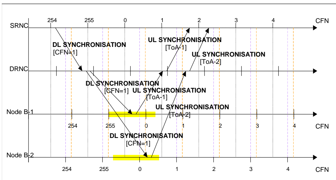
Figure 14: [FDD - TOA monitoring through FP Synchronisation Procedure during soft handover with selection/recombining in the DRNC]
