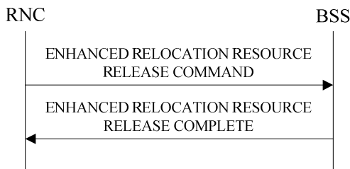
Figure 4D: Enhanced Relocation Resource Release Procedure, Successful Operation
