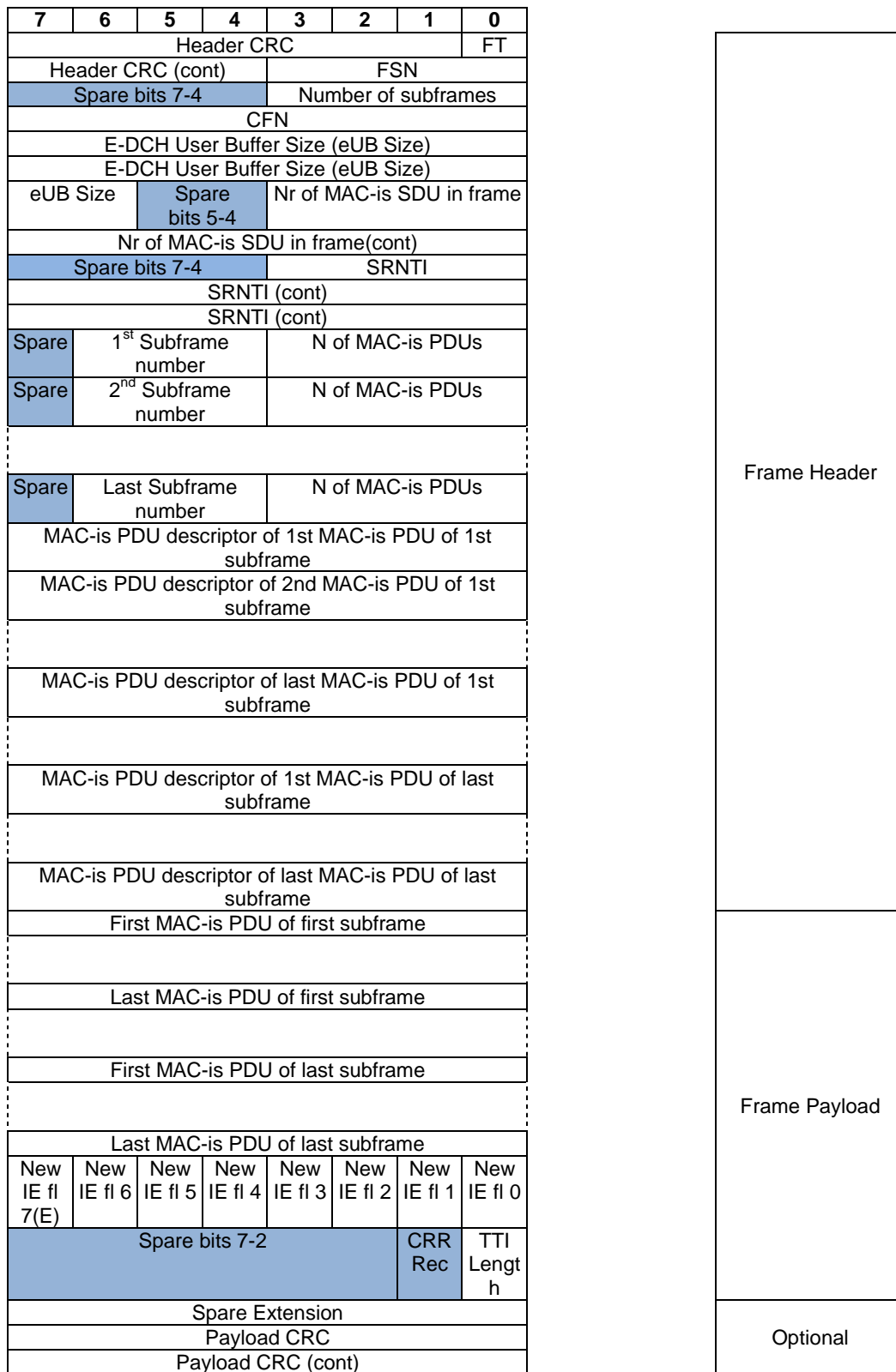
Figure 12C: E-DCH DATA FRAME structure
