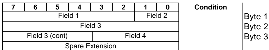
Figure 8: Example frame structure
