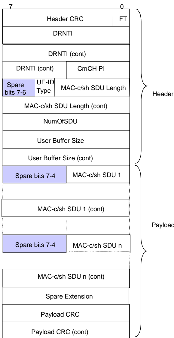
Figure 10: FACH DATA FRAME structure
