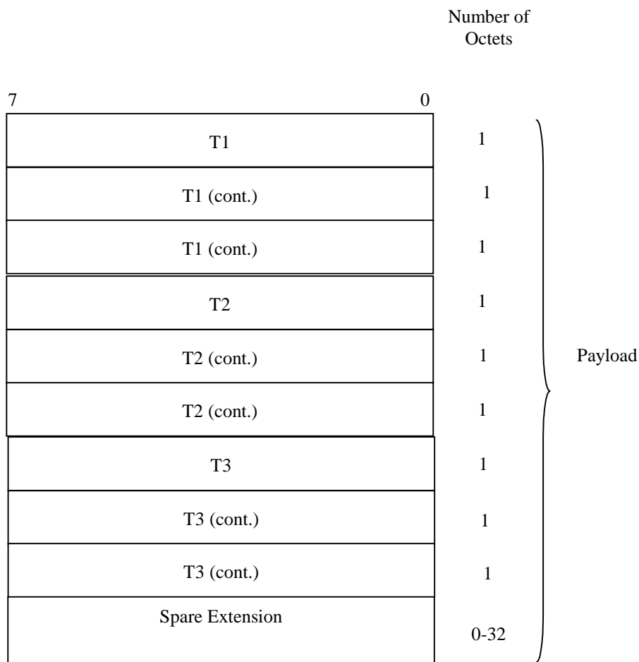
Figure 21: Structure of the payload for UL NODE SYNCHRONISATION control frame
