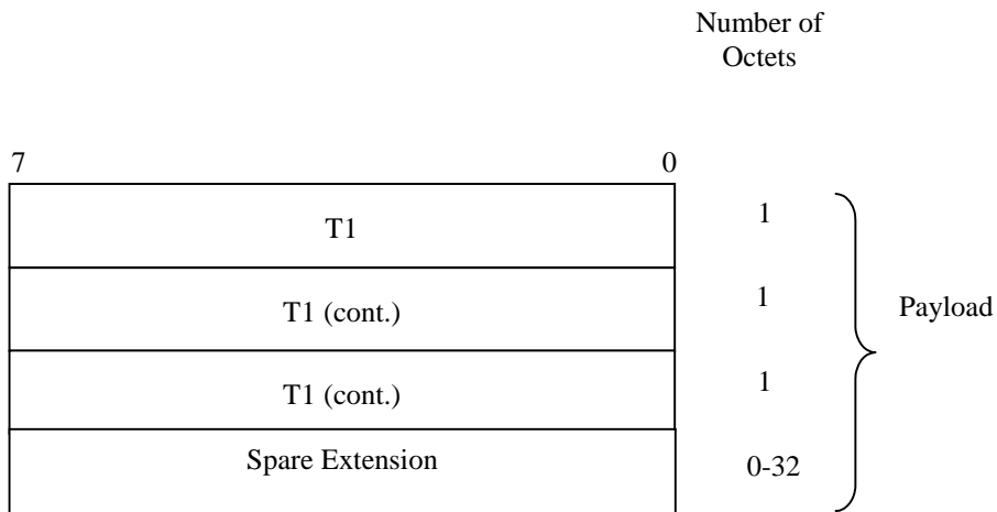
Figure 20: Structure of the payload for the DL NODE SYNCHRONISATION control frame
