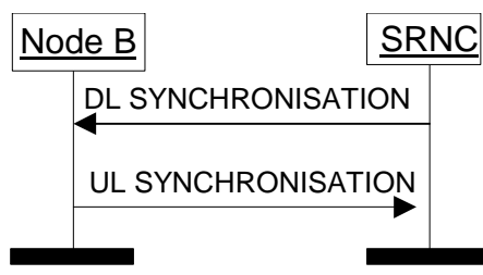
Figure 4: DCH Synchronization procedure
