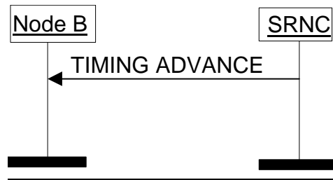
Figure 9A: Timing Advance procedure
