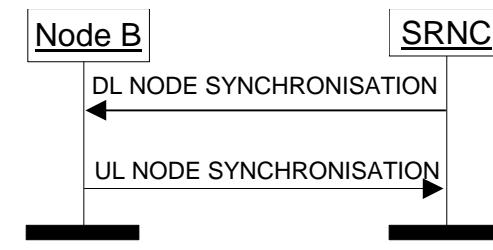
Figure 6: Node Synchronisation procedure
