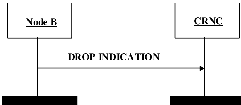
Figure 12E: HS-DSCH DROP INDICATION procedure
