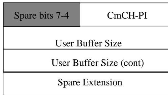
Figure 35: CAPACITY REQUEST payload structure
