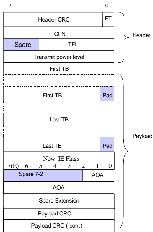
Figure 17: FACH DATA FRAME structure
