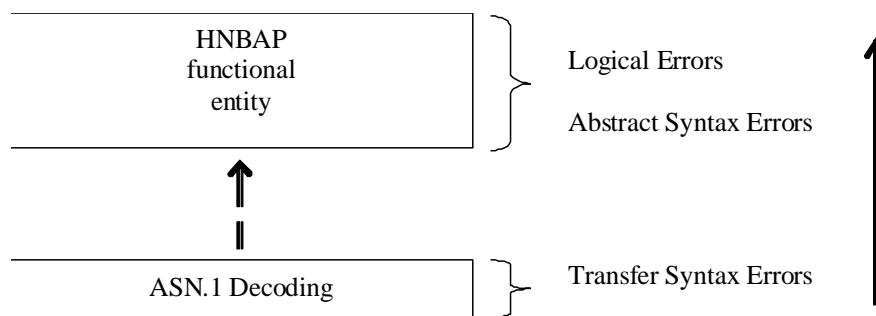
Figure 11: Protocol Errors in HNBAP
