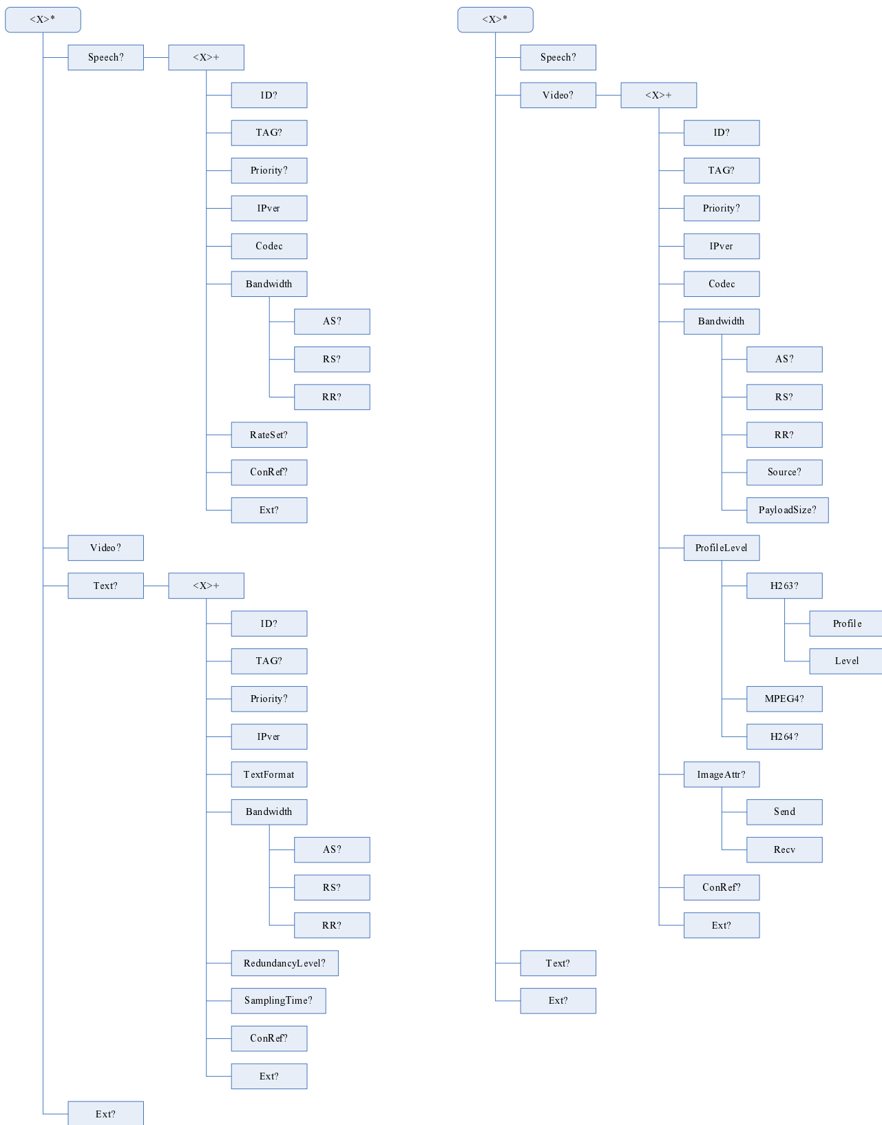
Figure 15.1: MTSI network preference management object tree
