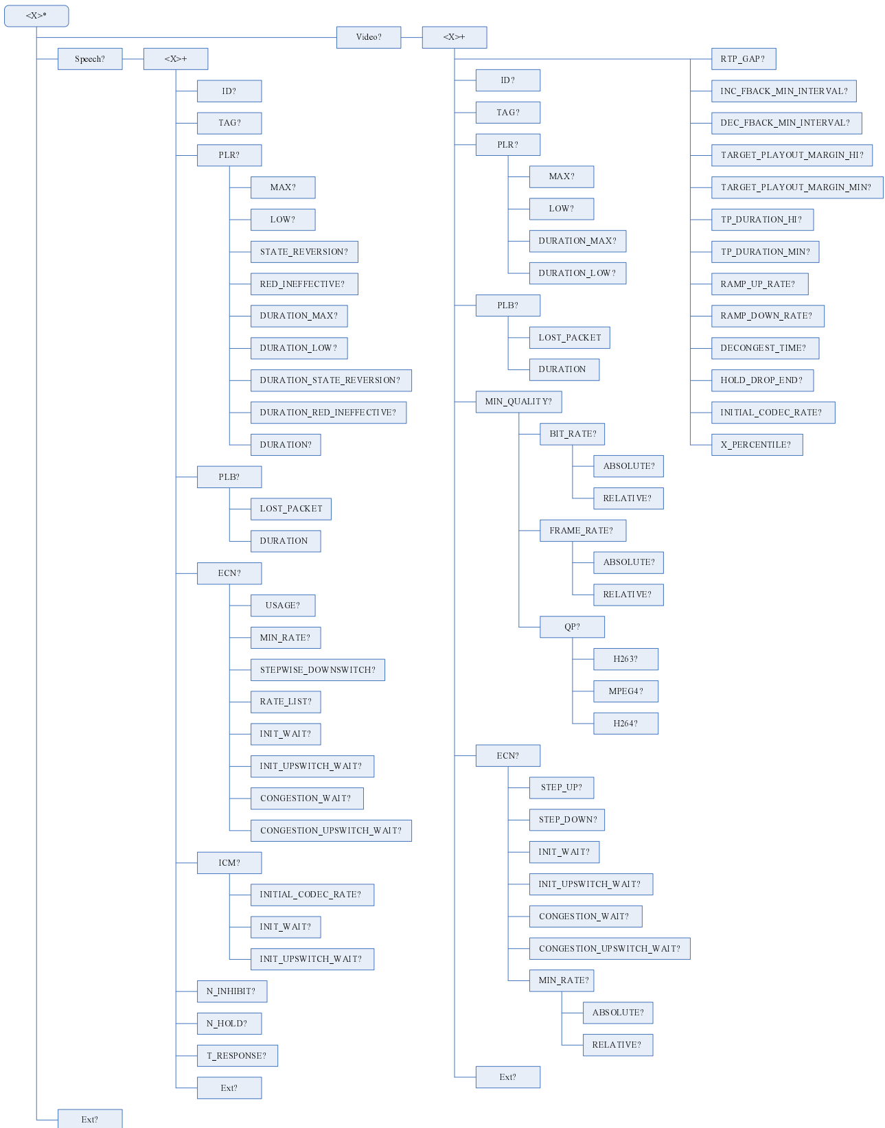
Figure 17.1: MTSI media adaptation management object tree
