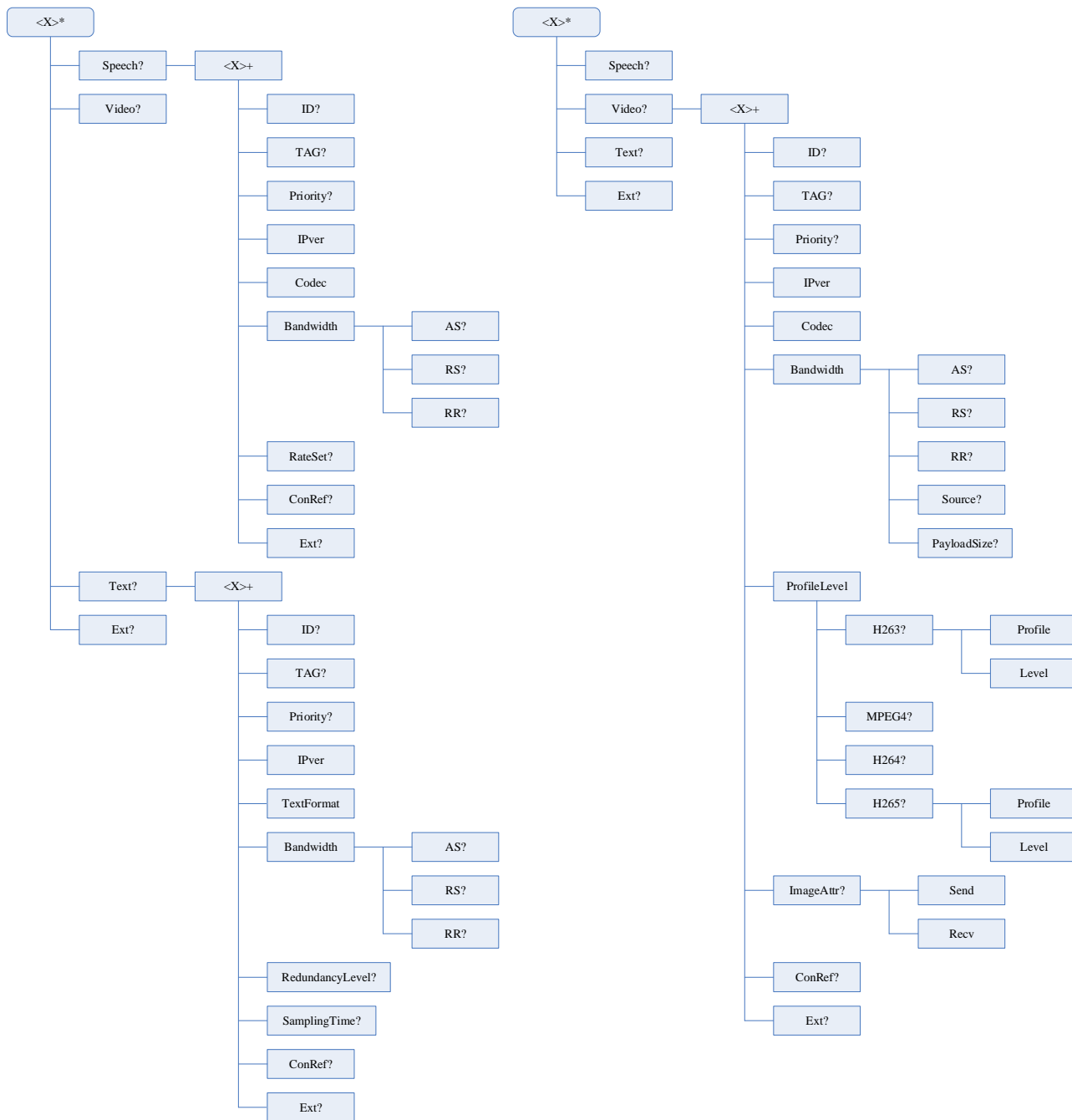
Figure 15.1: MTSI network preference management object tree
