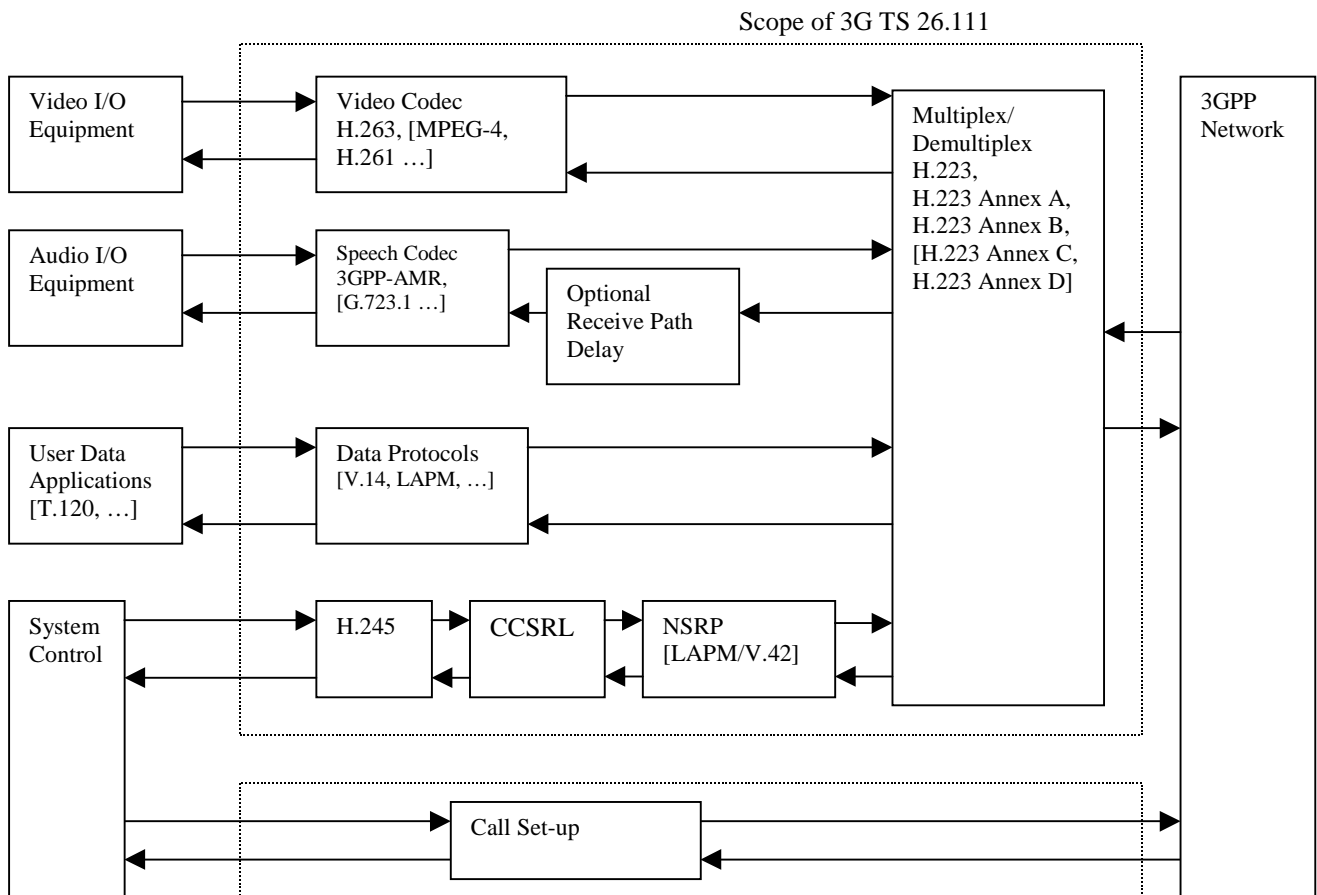
Figure 1 Scope of circuit switched multimedia 3GPP specification. Items in [brackets] are optional.
