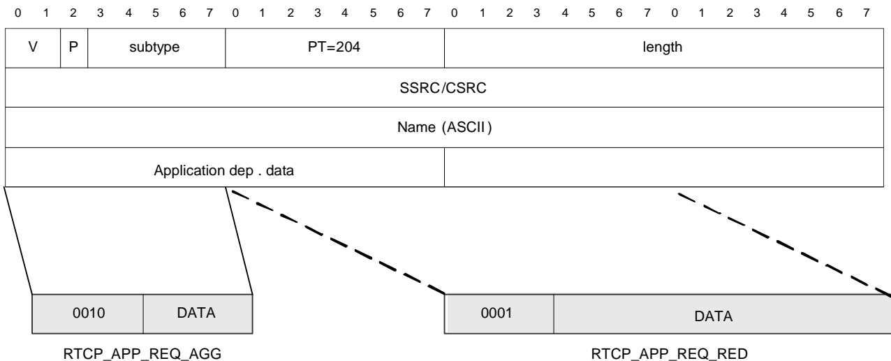
Figure 10.1: RTCP-APP formatting
