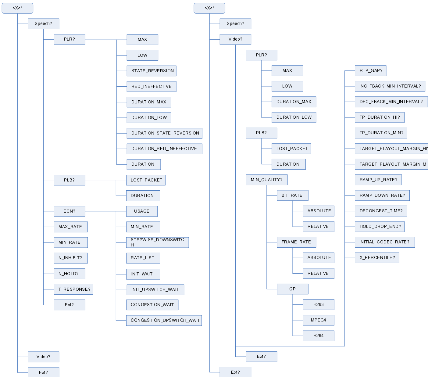
Figure 17.1: MTSI media adaptation management object tree
