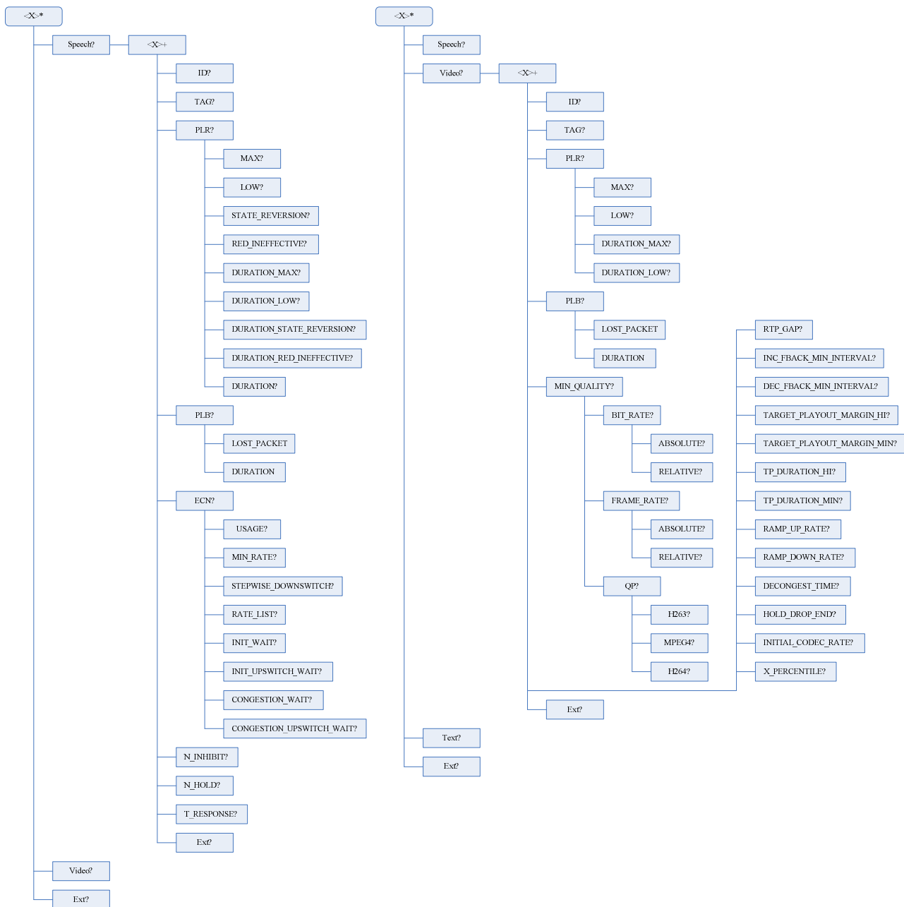
Figure 17.1: MTSI media adaptation management object tree
