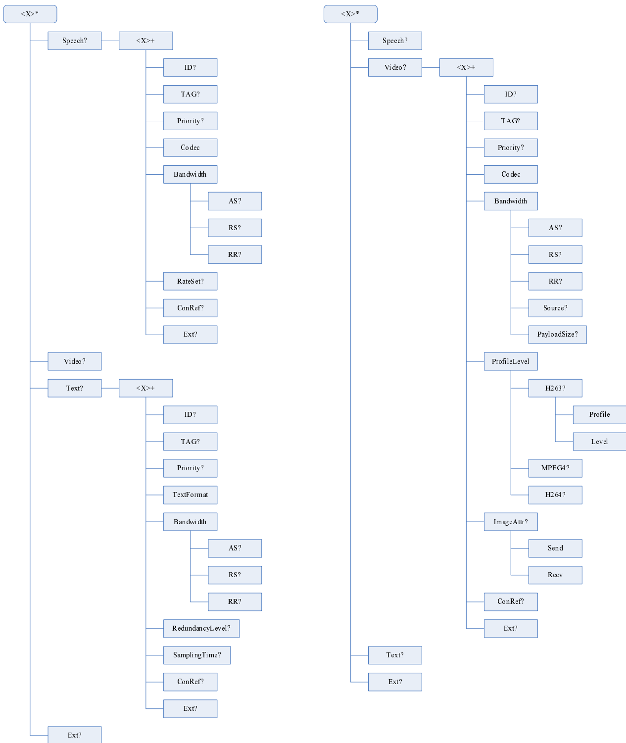
Figure 15.1: MTSI network preference management object tree
