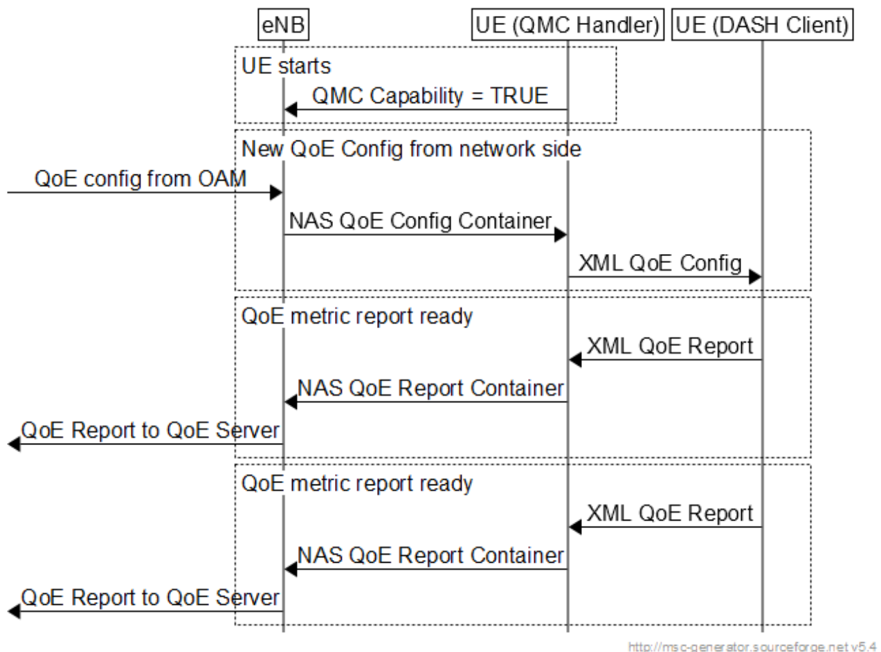
Figure L-1: example signalling diagram
