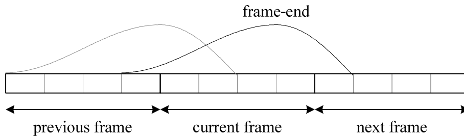
Figure 86: Relative positions and length of the LP analysis windows for the AMR-WB interoperable option
