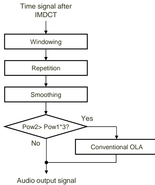
Figure14: Block diagram of repetition & smoothing method for erased frame
