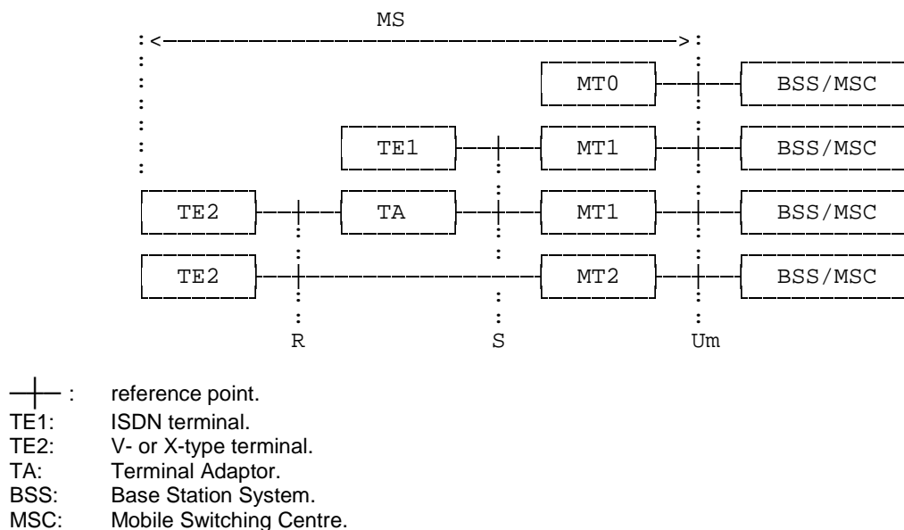
Figure 1: A/Gb mode PLMN Access Reference Configuration
