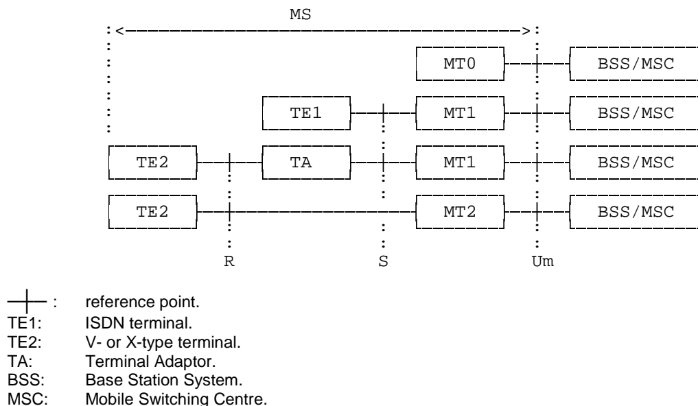
Figure 1: A/Gb mode PLMN Access Reference Configuration
