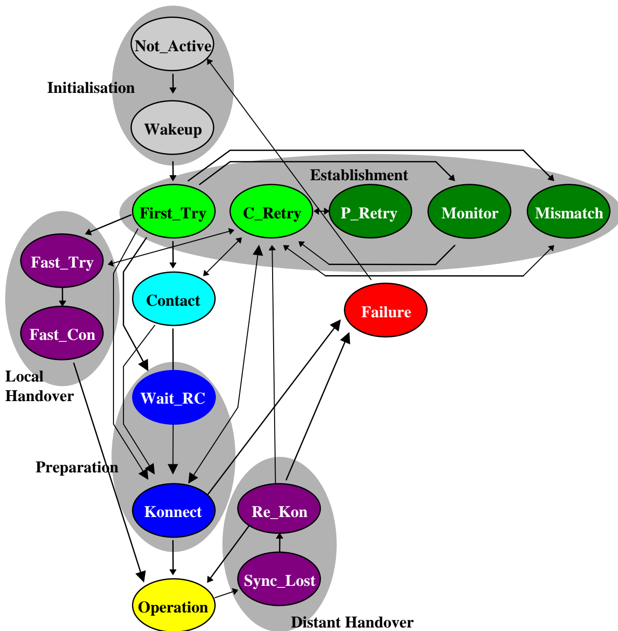
Figure 9-1: TFO_Protocol State Machine with most important transitions
