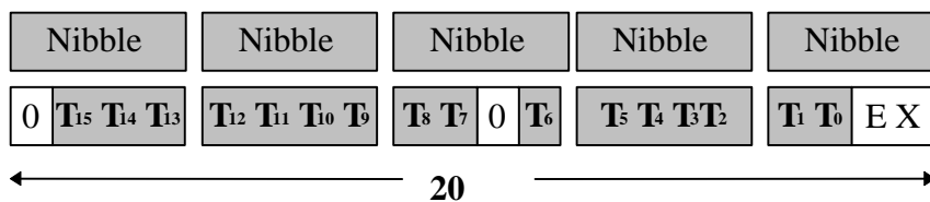
Figure A.2.3-2: IPE_Mode_Extension_Block for the IS_IPE Message
