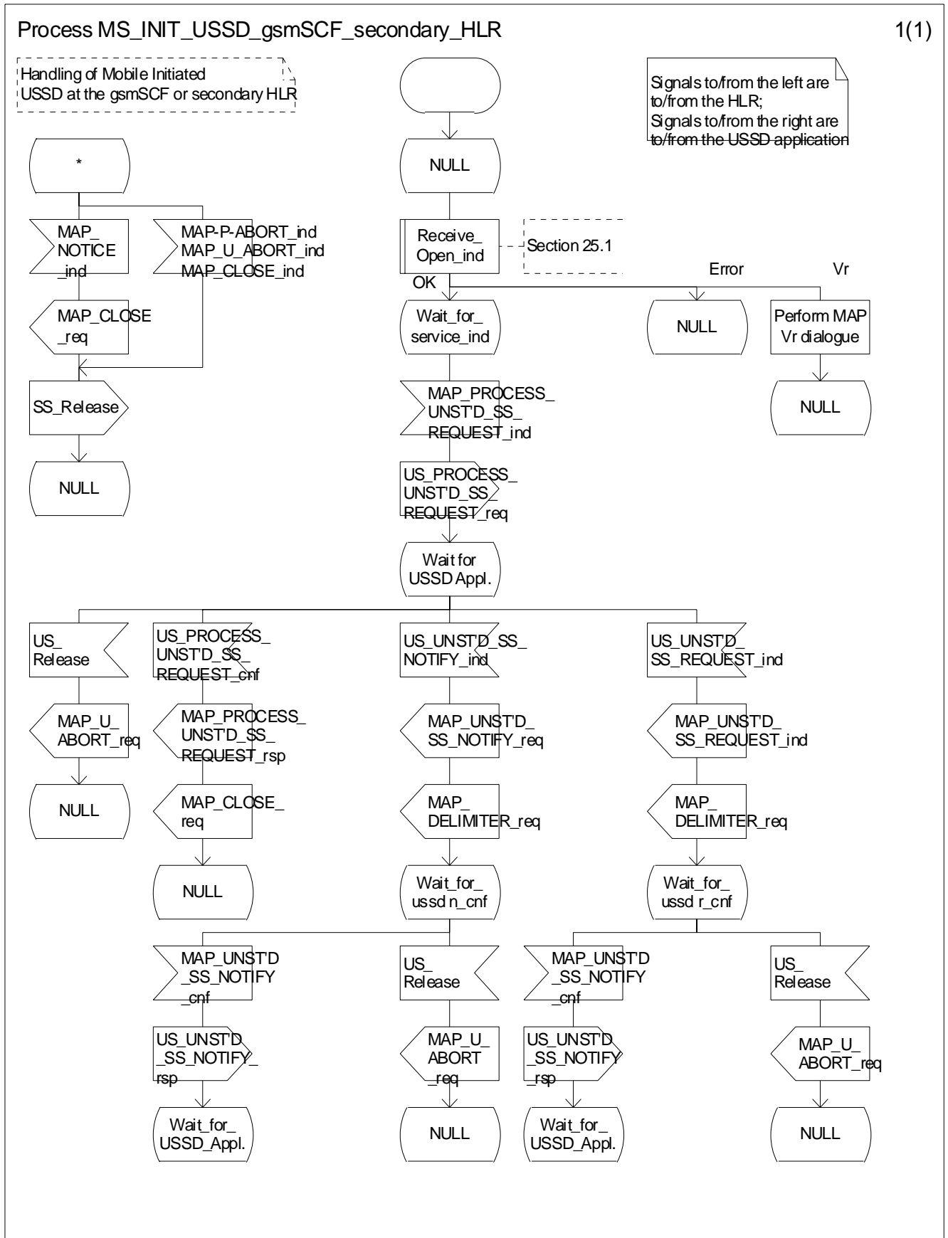
Figure 22.9.5/1 Process MS_INIT_USSD_gsmSCF_secondary_HLR
