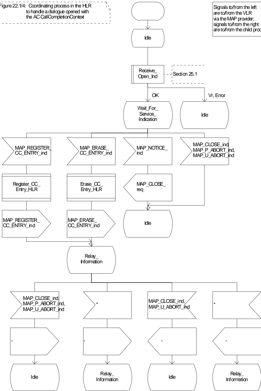
Figure 22.1/4: Process_CC_Coord_HLR
