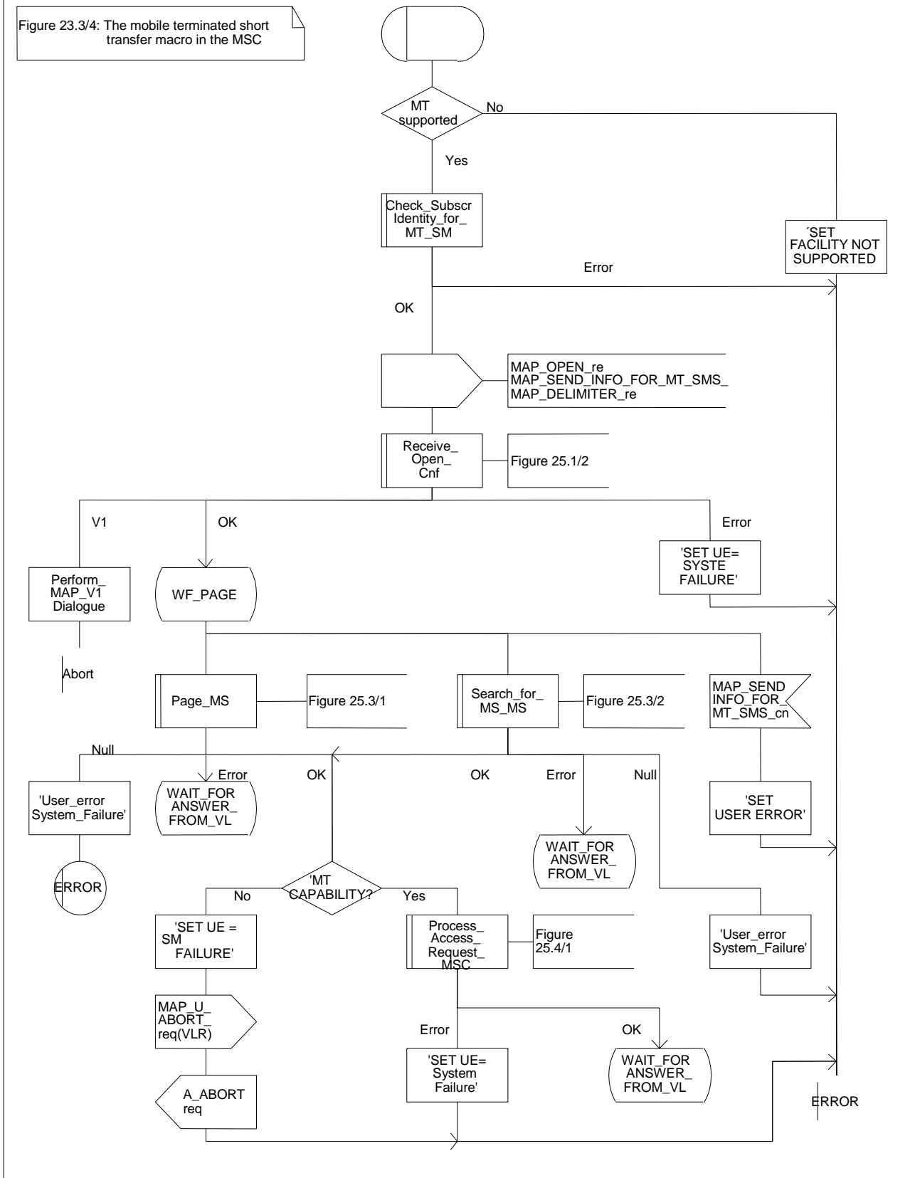
Figure 23.3/4 (sheet 1 of 4): Macro MT_SM_Transfer_MSC
