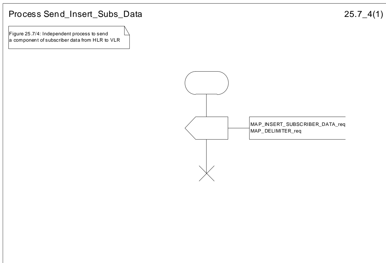
Figure 25.7/4: Process Send_Insert_SubData
