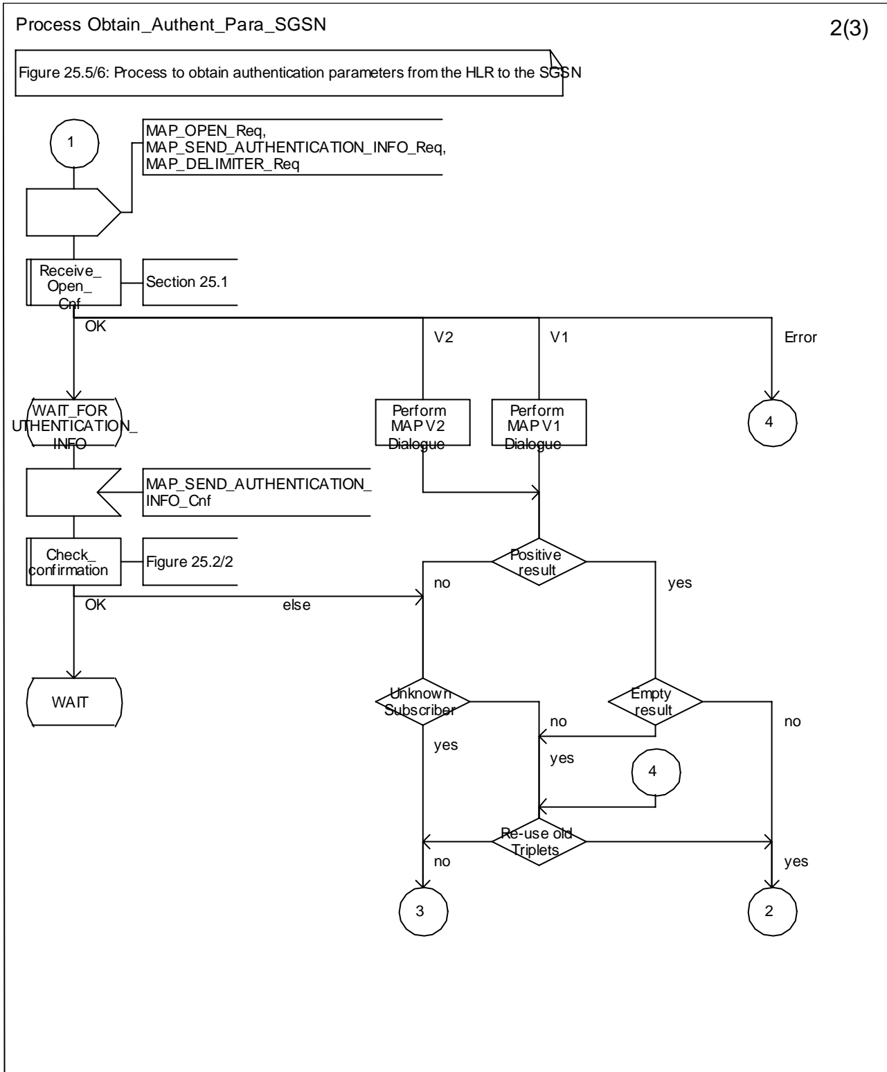
Figure 25.5/6 (sheet 2 of 3): Process Obtain_Authen_Para_SGSN
