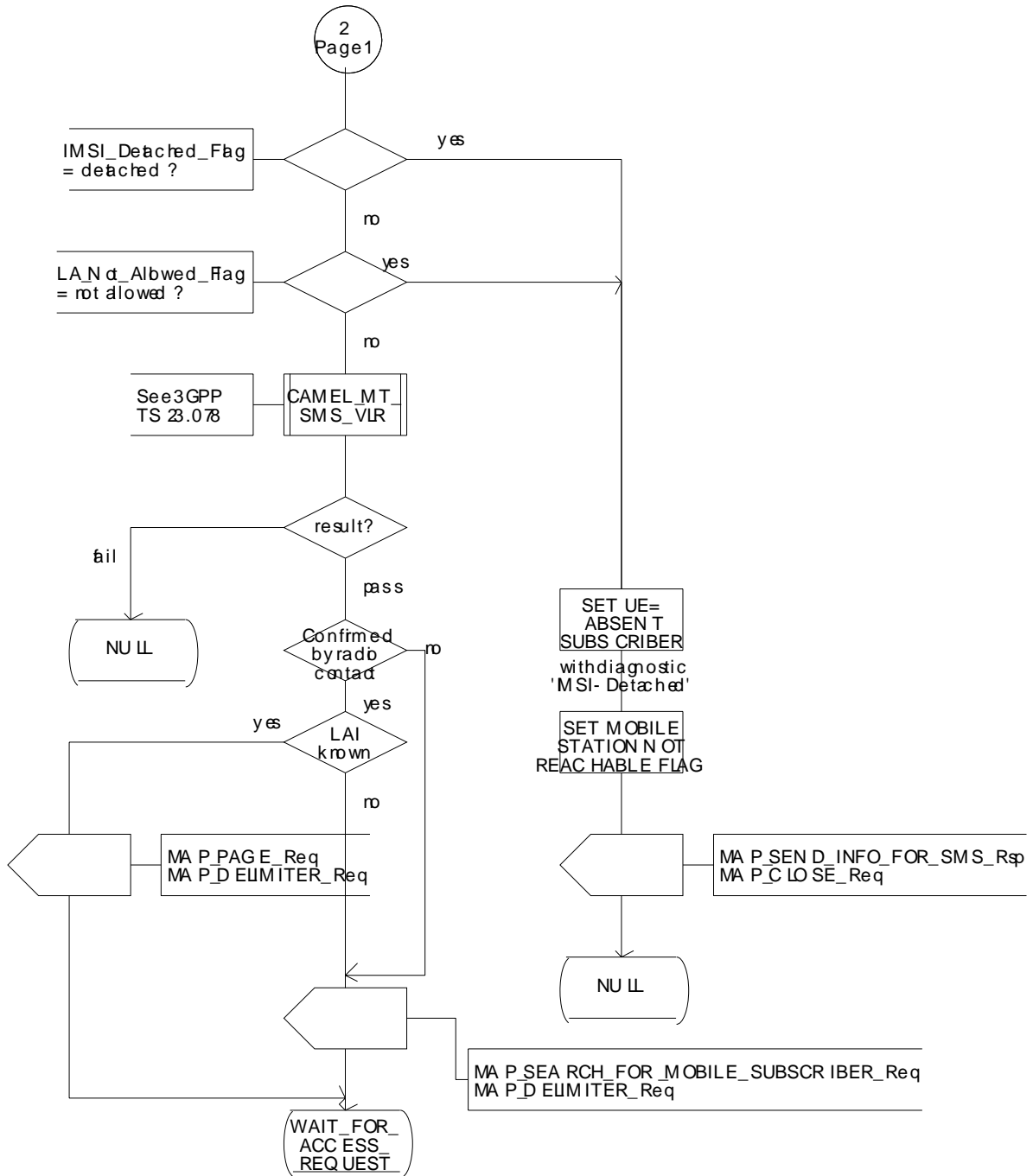
Figure 23.3/5 (sheet 2 of 3): Process MT_SM_VLR
