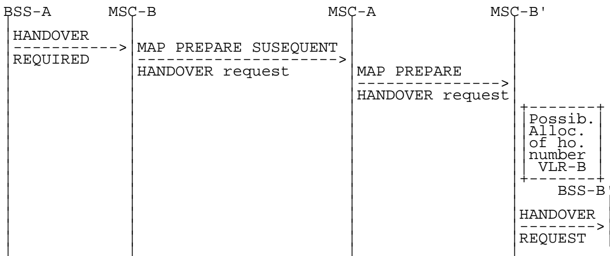
Figure 16: Signalling for Subsequent Inter-MS-C Handover to third MS-C (MS-B') initiation
