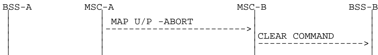
Figure 10: Signalling for Basic Inter-MSC Handover completion (Negative outcome)
