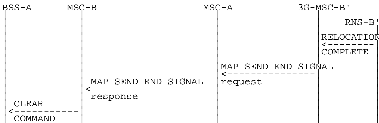
Figure 48: Signalling for Subsequent Inter-MSC Handover to third MSC (3G_MSC-B') completion (Successful completion of the procedure)
