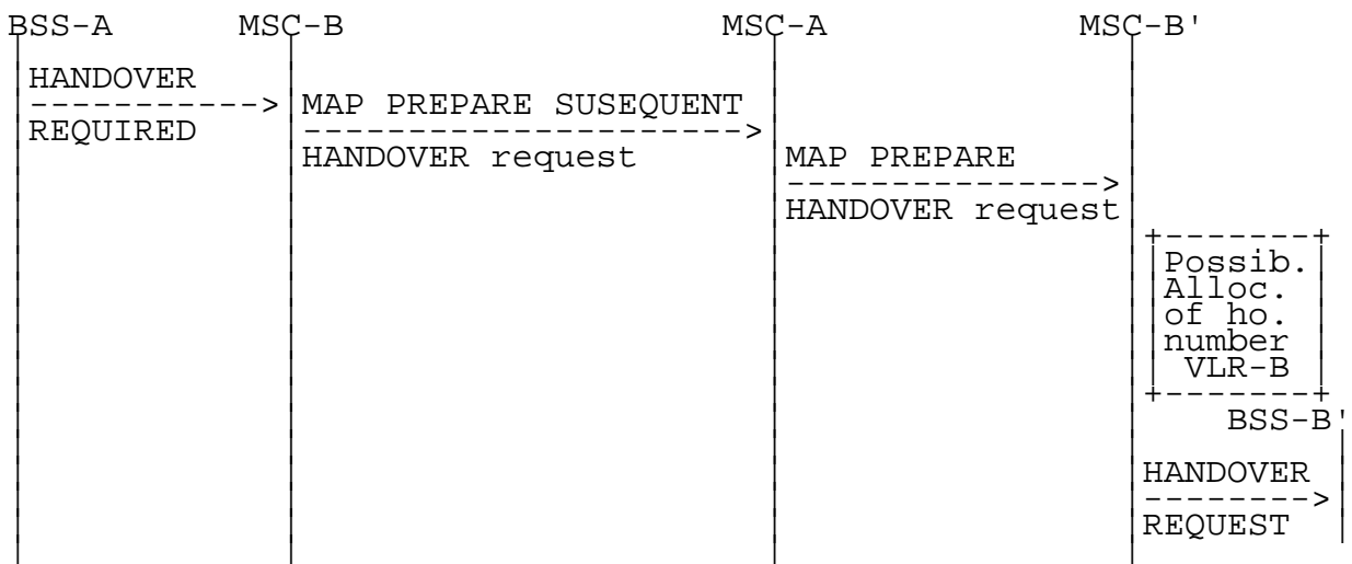
Figure 16: Signalling for Subsequent Inter-MSK Handover to third MSC (MSC-B') initiation
