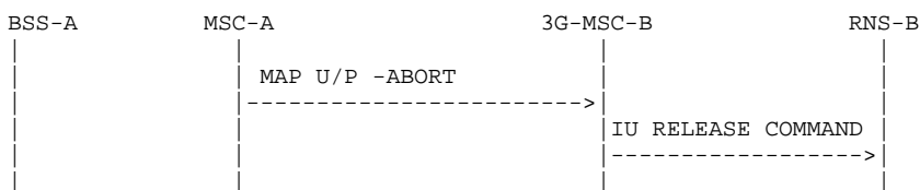
Figure 42: Signalling for Basic Inter-MS-C Handover completion (Negative outcome)
