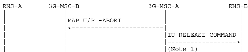
Figure 59: Signalling for Subsequent Inter-MSB Relocation back to 3G_MSC-A completion (Unsuccessful completion of the procedure)
