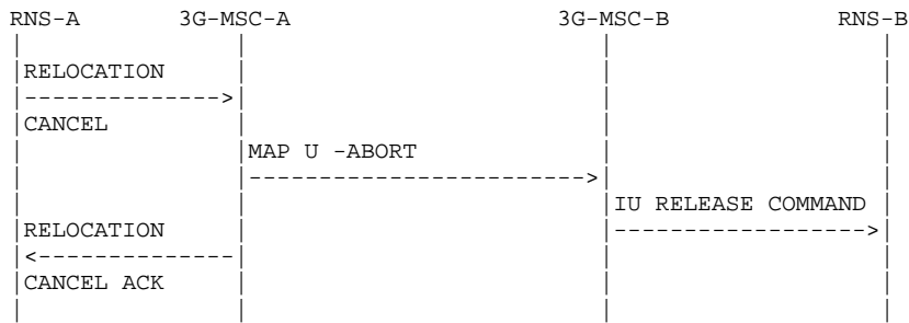
Figure 51: Signalling for Basic Inter-MSA Relocation execution (Negative outcomes)
