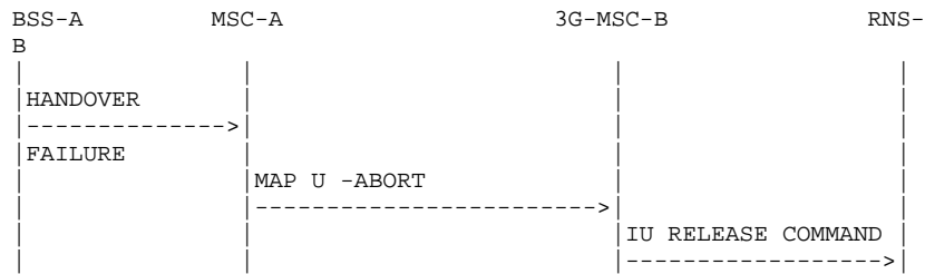
Figure 39: Signalling for Basic Inter-MS-C Handover execution (Negative outcomes)
