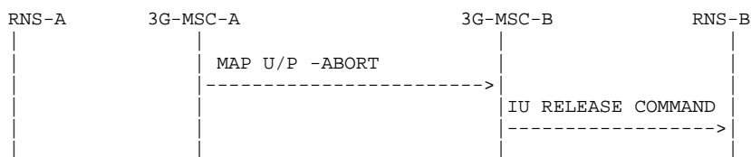
Figure 54: Signalling for Basic Inter-MSA Relocation completion (Negative outcome)
