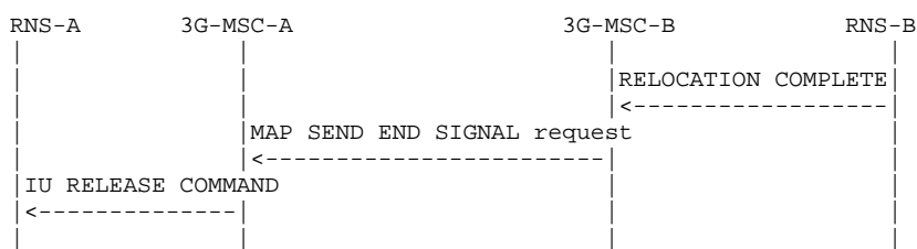
Figure 52: Signalling for Basic Inter-MSA Relocation completion
