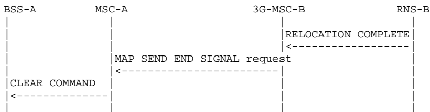
Figure 40: Signalling for Basic Inter-MS-C Handover completion
