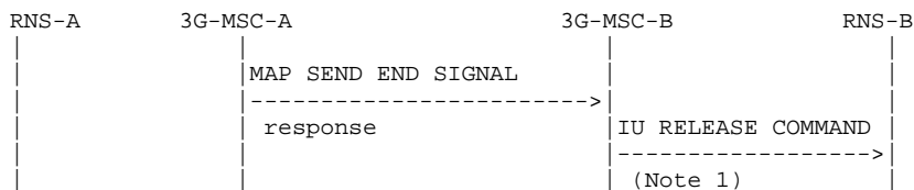
Figure 53: Signalling for Basic Inter-MSA Relocation completion (Positive outcome)
