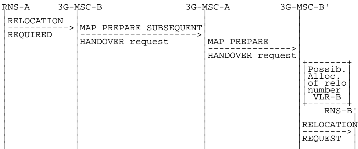
Figure 60: Signalling for Subsequent Inter-MSR Relocation to third MSR (3G_MSC-B') initiation
