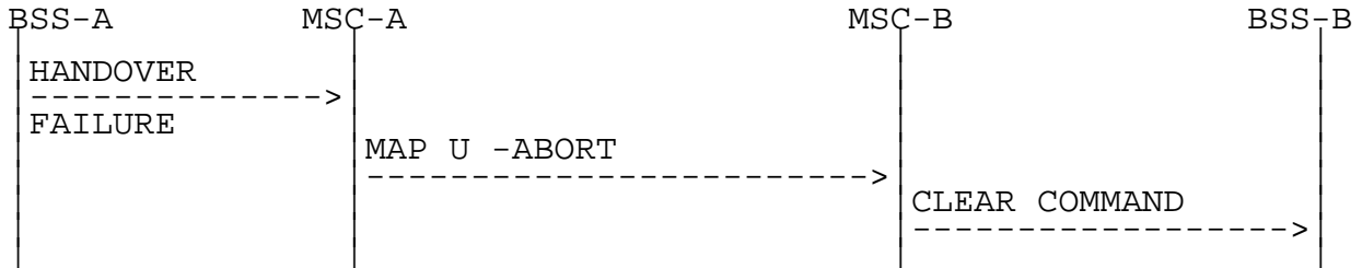
Figure 7: Signalling for Basic Inter-MSC Handover execution (Negative outcomes)
