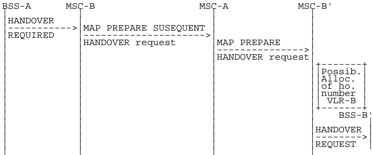
Figure 16: Signalling for Subsequent Inter-MSB Handover to third MSB (MSB-B') initiation
