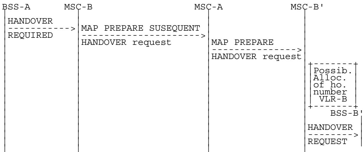
Figure 16: Signalling for Subsequent Inter-MSB Handover to third MSB (MSC-B') initiation
