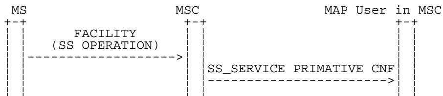
Figure 6.7: Signalling flow for Network Initiated SS operation return result
