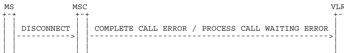
Figure 5.22: Signalling of a Call Deflection Request
