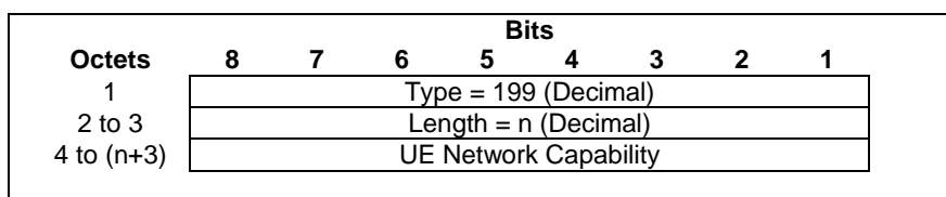
Figure 7.7.99: UE Network Capability Information Element
