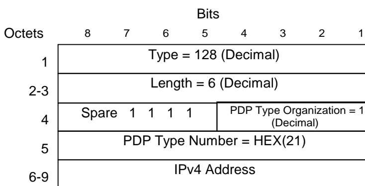
Figure 36: End User Address Information Element for IPv4
