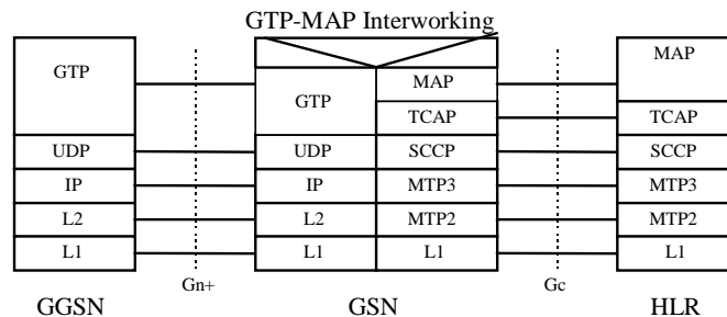
Figure 7: GGSN - HLR Signalling via a GTP-MAP Protocol-Converter in a GSN
