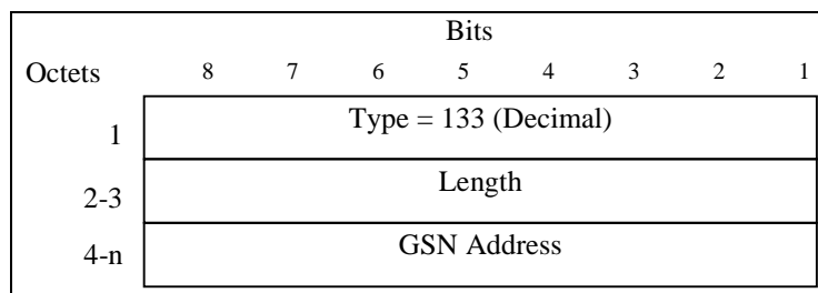
Figure 46: GSN Address Information Element
