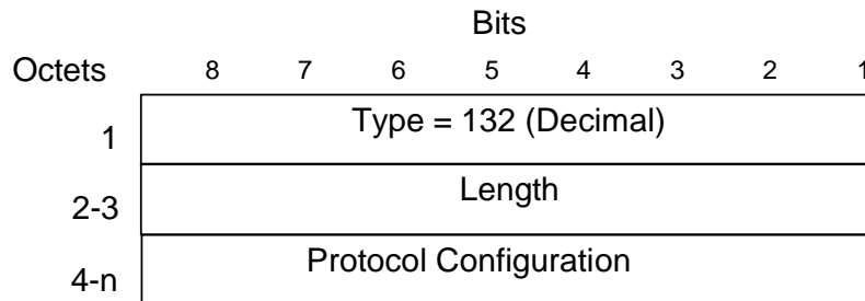
Figure 45: Protocol Configuration Options Information Element
