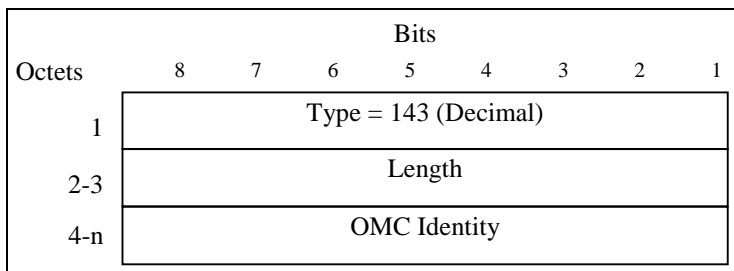
Figure 57: OMC Identity Information Element
