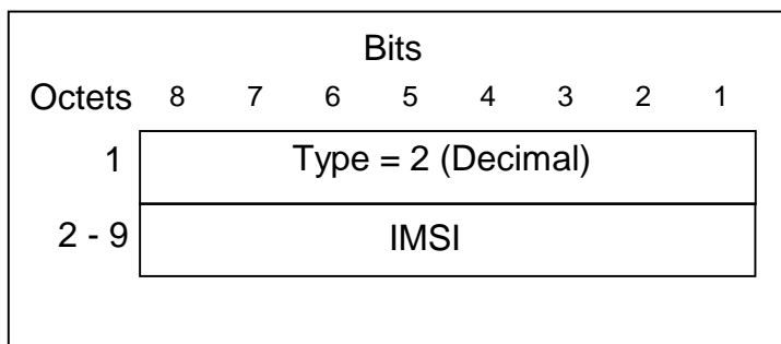
Figure 10: IMSI Information Element
