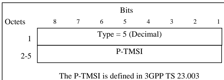
Figure 13: The Packet TMSI Information Element
