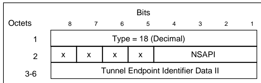
Figure 23: Tunnel Endpoint Identifier Data II Information Element
