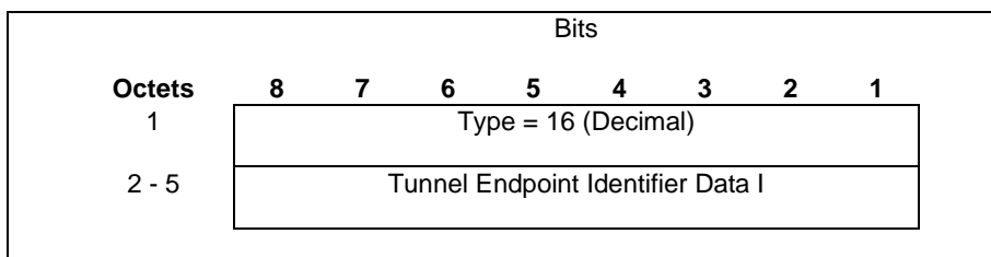
Figure 21: Tunnel Endpoint Identifier Data I Information Element
