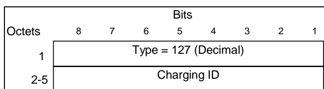
Figure 34: Charging ID Information Element
