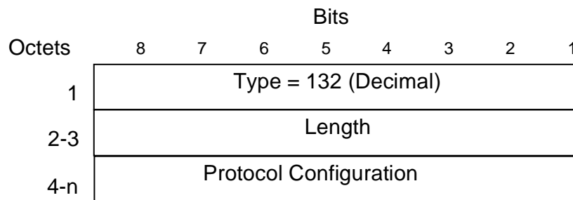
Figure 45: Protocol Configuration Options Information Element
