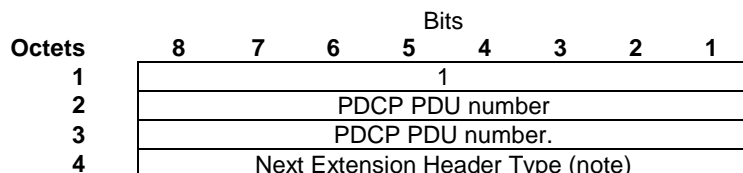
Figure 6: PDCP PDU number Extension Header
