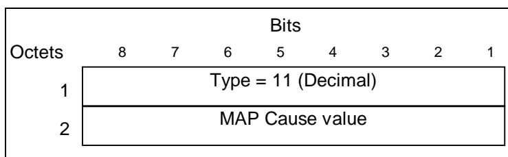
Figure 16: MAP Cause Information Element
