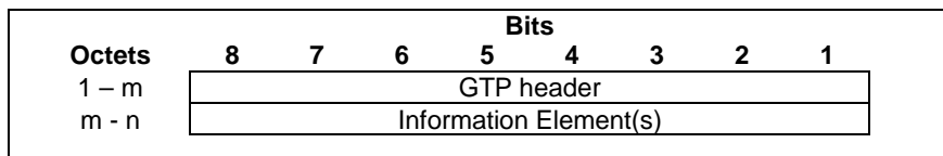
Figure 64: GTP Header followed by subsequent Information Elements
