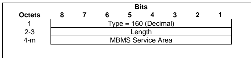
Figure 7.7.60.1: MBMS Service Area Information Element
