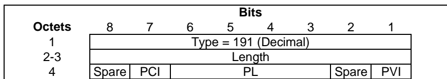
Figure 7.7.91.1: Evolved Allocation/Retention Priority Information Element
