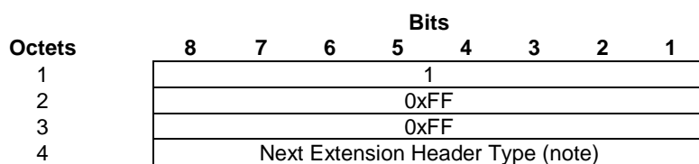
Figure 8: Suspend Response Extension Header
