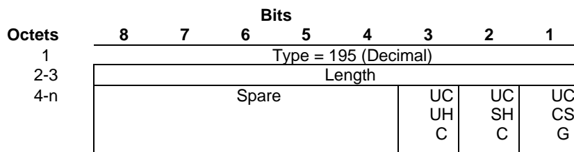
Figure 7.7.95.1: User CSG Information
